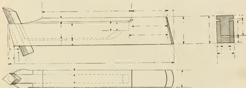
UNIQUE TOOL HOLDER.
